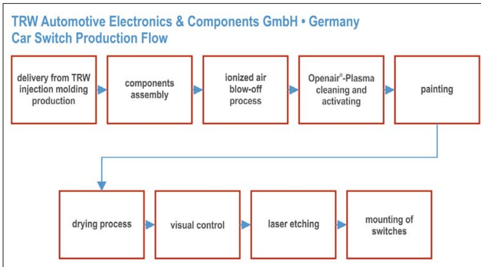
Flow diagram of switch production including the painting process. (All images Plasmatreat)
